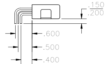
TERMINAL TYPE 7 FINISH: CASE-TIN PLATED TERMINALS-TIN/LEAD
