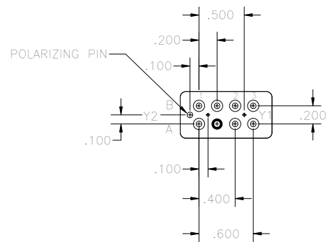
TERMINAL TYPE 7 FINISH: CASE-TIN PLATED TERMINALS-TIN/LEAD
