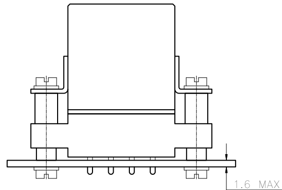
MOUNTING
